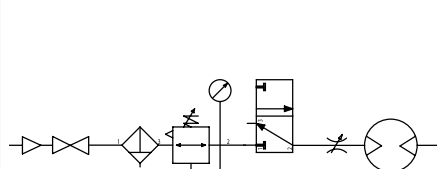
Shut-off, filtering, pressure regulation and control valve
