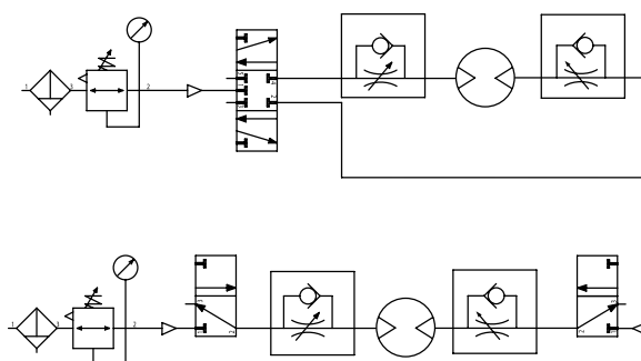
Reversible motor with 5/3 control valve
